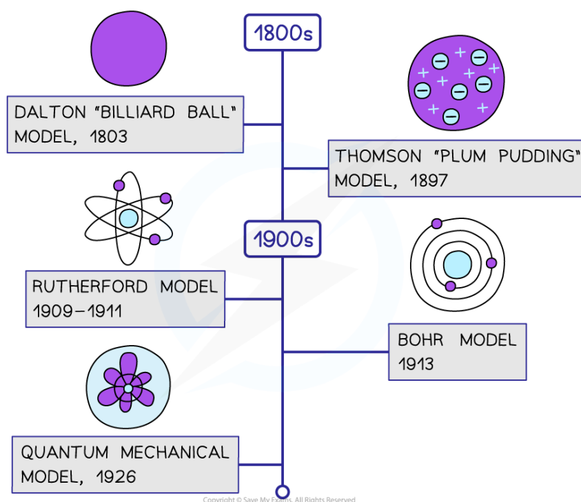
Timeline of the changing models of the atom
