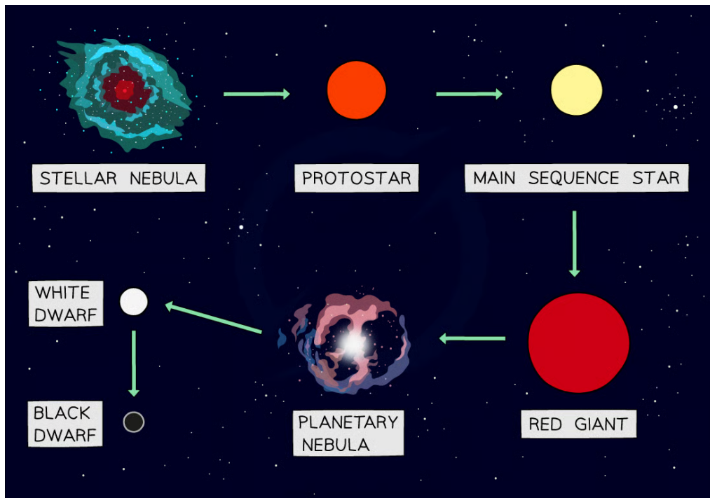
The lifecycle of a low mass star
