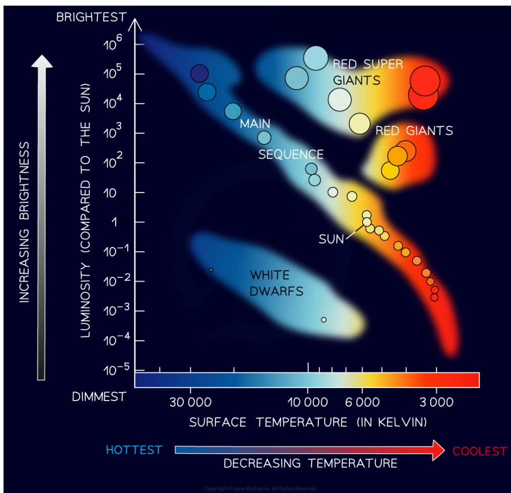
The Hertzsprung–Russell Diagram
